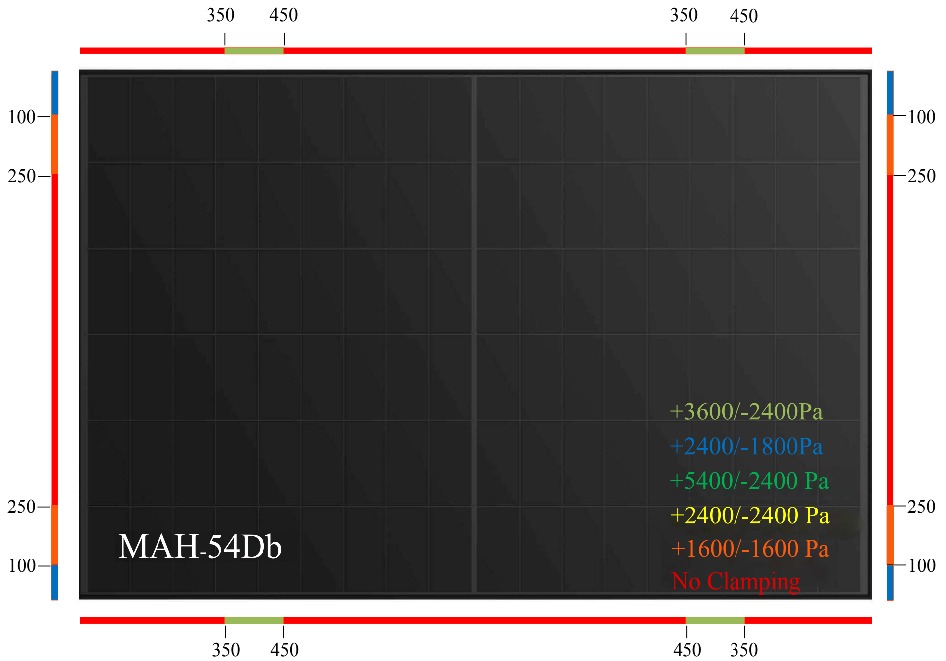
This load graph present when the purlin overlap the long side/short side, number means the distance between the edge of clamp to the frame. Unit:mm
