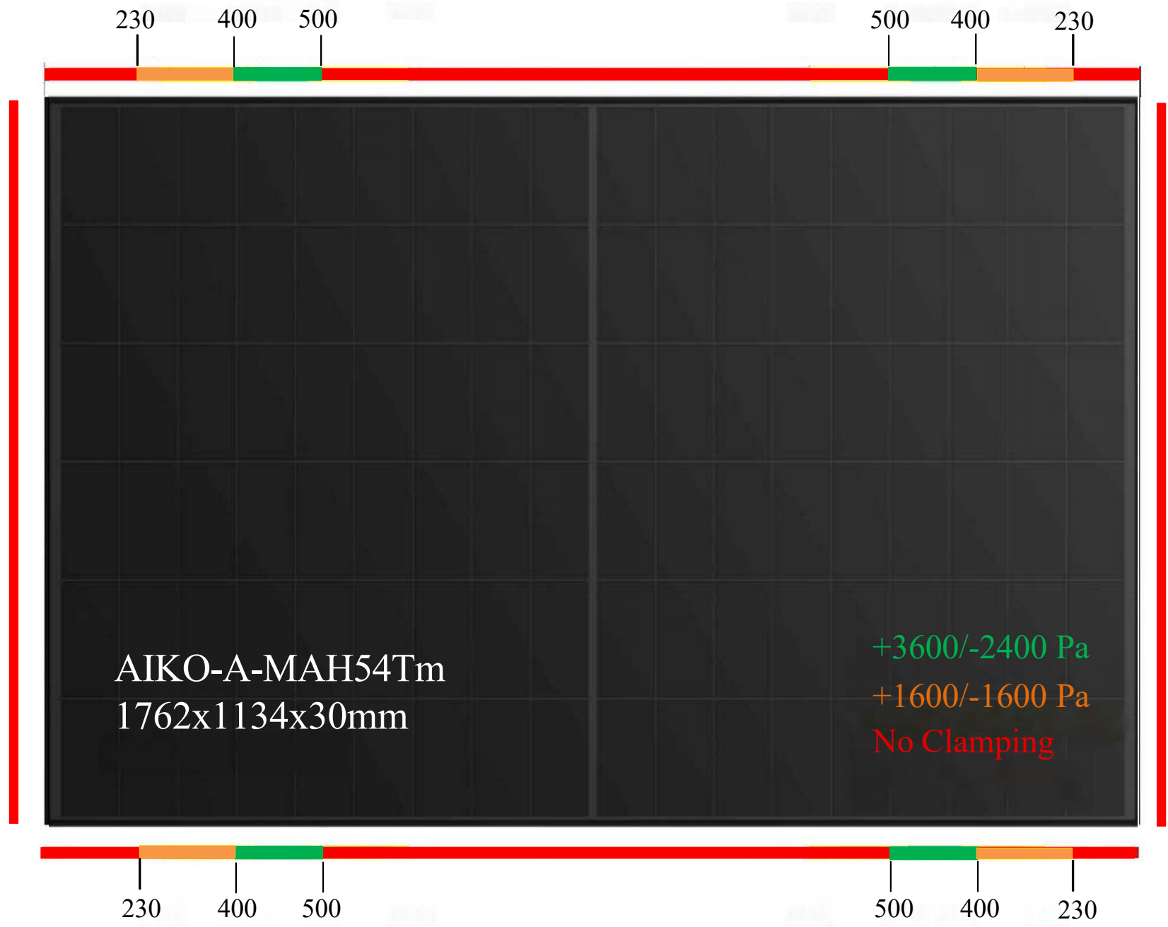
This load graph present when the purlin cross the long side/short side, number means the distance between the edge of clamp to the frame. Unit:mm
